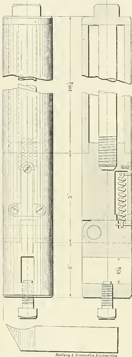
SLOTTER BAR, SANTA FE SHOPS.
